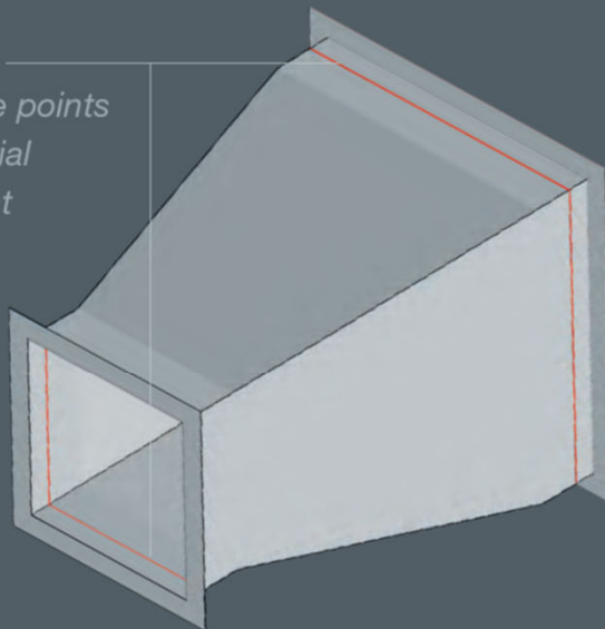
Conventional Ducting
